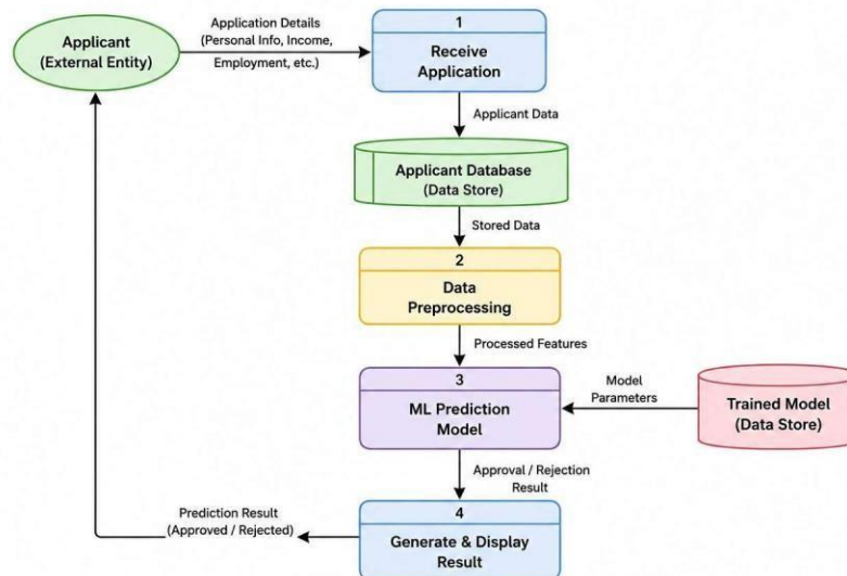
Data Flow Diagram (Credit Card Approval Prediction System)
